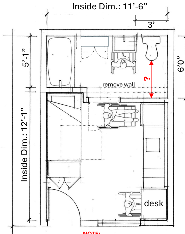
ADA Studio (216 sf, gross)
